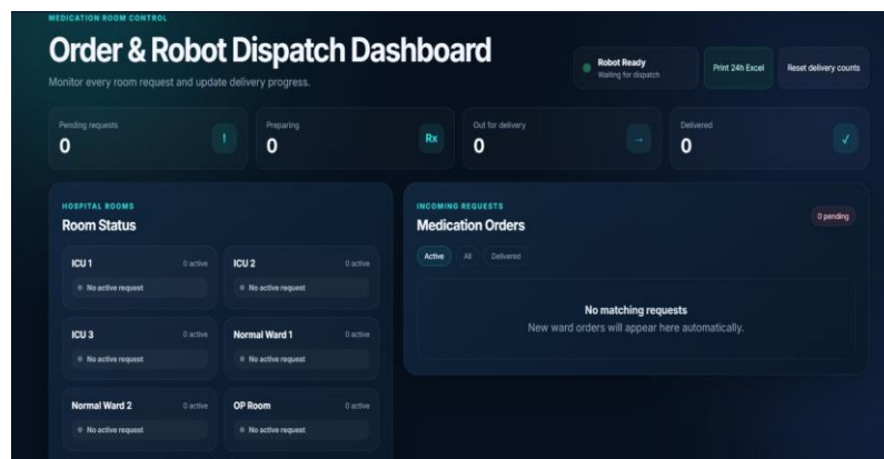
Figure 6.1 Website Overview
