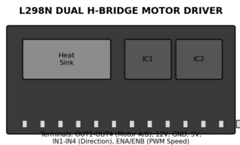
Figure 3.2.4 L298N Motor Driver
