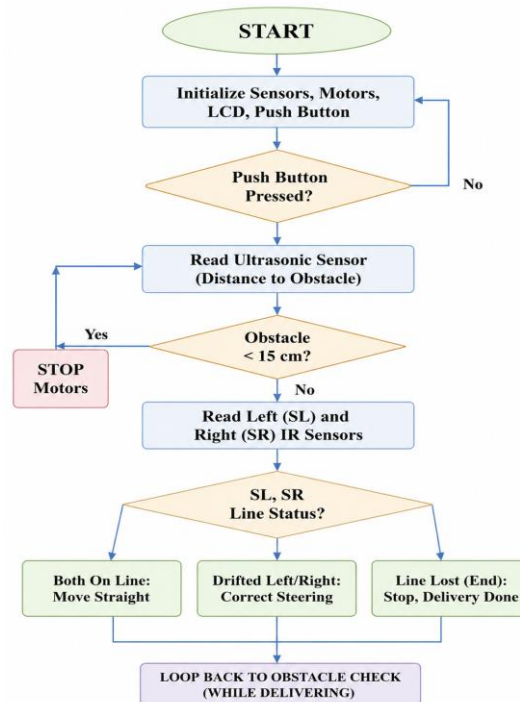
Figure 4.8 Control Algorithm Flowchart
